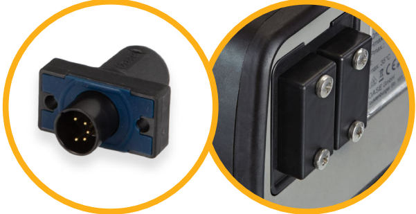
An End Resistor in the last device signals the end of the run to the Cloud Controller
